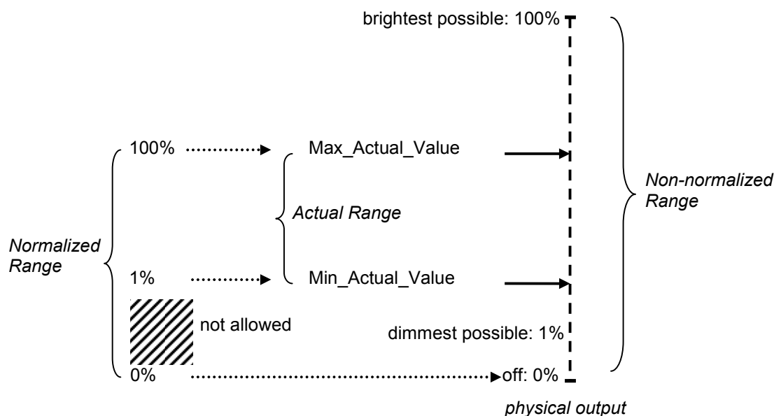
Figure 12-X1. Normalized Range of the Lighting Output
