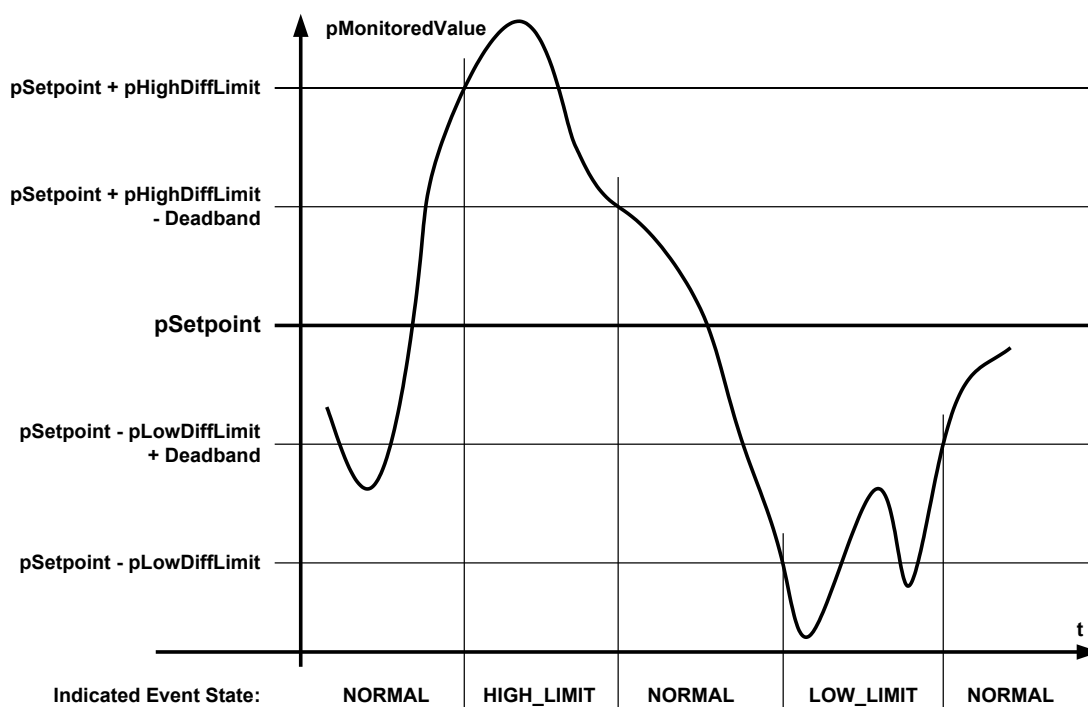
Figure 13-Y5 shows the relationship of the various parameters used in the FLOATING_LIMIT algorithm. In this figure, pTimeDelay is assumed to have a value of zero.
