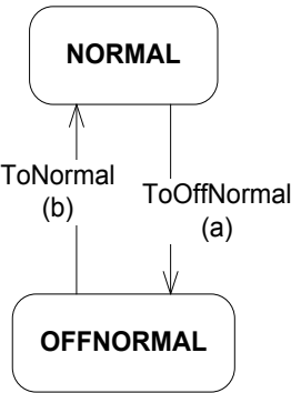
Figure 13-Y4. Transitions indicated by COMMAND_FAILURE algorithm
