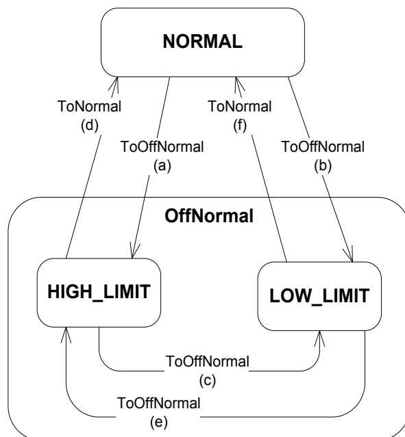
Figure 13-Y6. Transitions indicated by FLOATING_LIMIT algorithm
