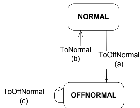
Figure 13-Y2. Transitions indicated by CHANGE_OF_STATE algorithm
