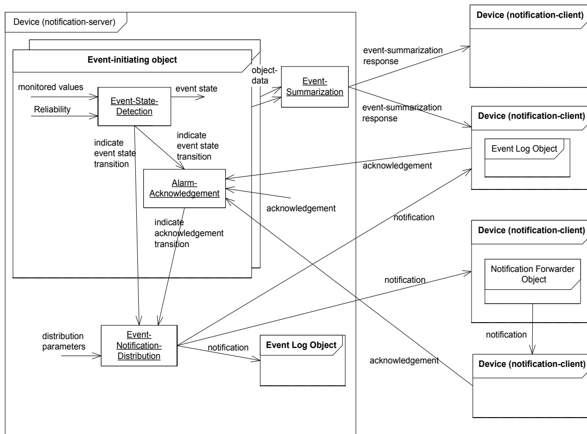
Figure 13-X1. Overview of the Event Detection and Reporting Model
