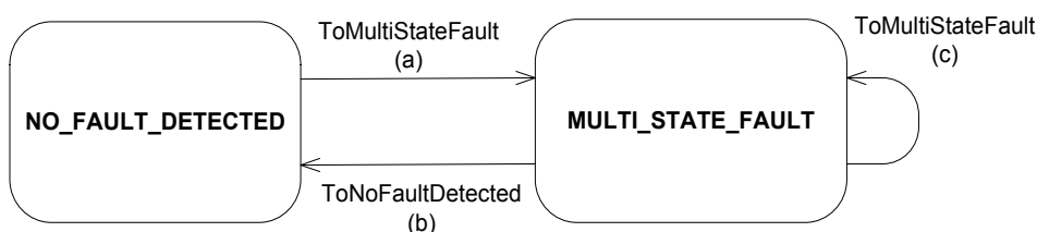
Figure 13-Y21. Transitions indicated by FAULT_STATE algorithm
