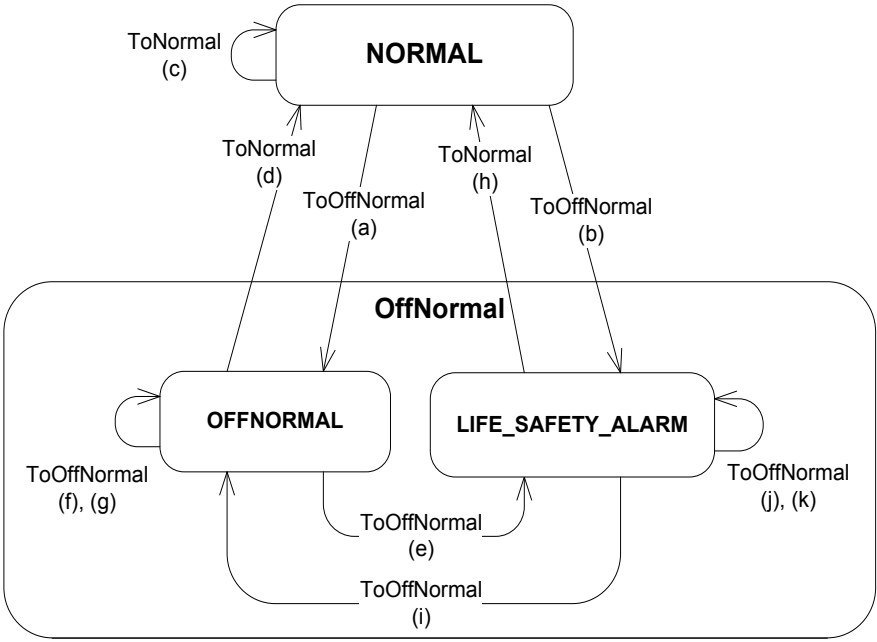
Figure 13-Y9. Transitions indicated by CHANGE_OF_LIFE_SAFETY algorithm
