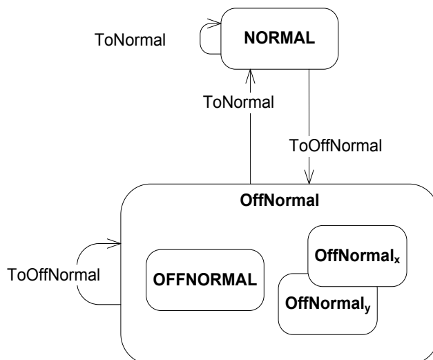
Figure 13-Y11. Transitions indicated by EXTENDED algorithm
