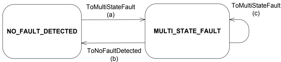
Figure 13-Y18: Transitions indicated by FAULT_CHARACTERSTRING algorithm
