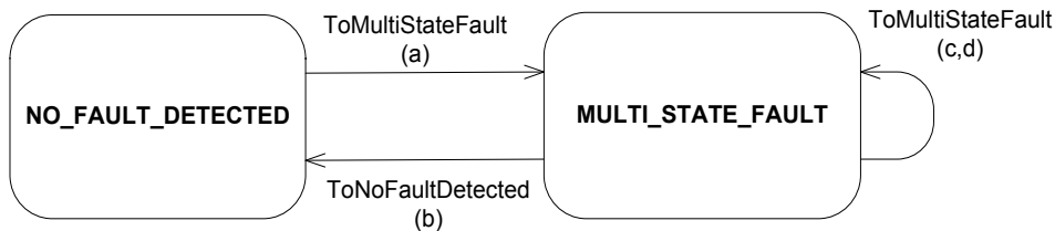
Figure 13-Y20. Transitions indicated by FAULT_LIFE_SAFETY algorithm
