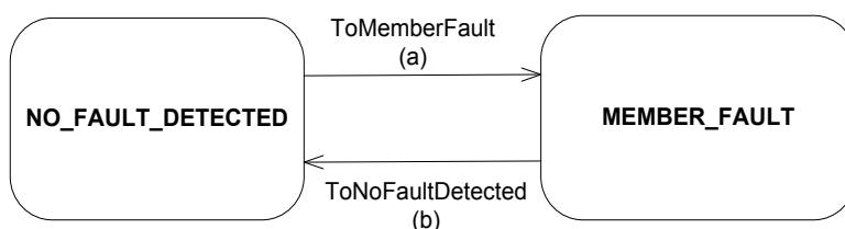
Figure 13-Y21. Transitions indicated by FAULT_STATUS_FLAGS algorithm
