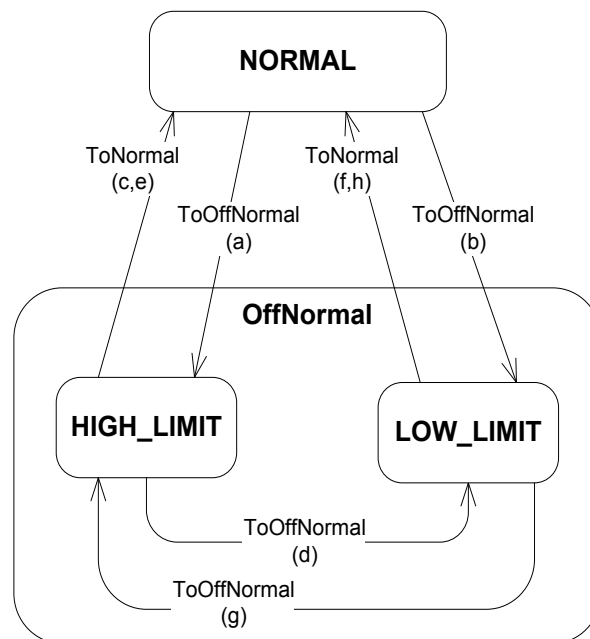
Figure 13-Y16. Transitions indicated by UNSIGNED_OUT_OF_RANGE algorithm
