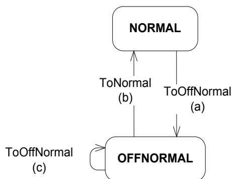
Figure 13-Y12. Transitions indicated by CHANGE_OF_STATUS_FLAGS algorithm
