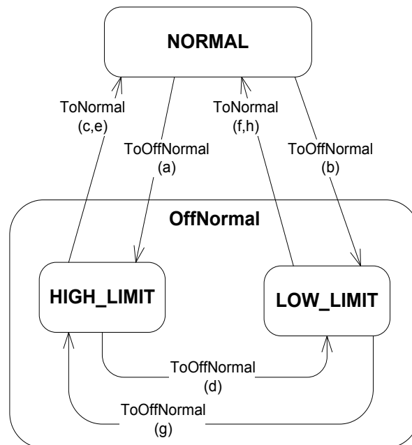
Figure 13-Y7. Transitions indicated by OUT_OF_RANGE algorithm
