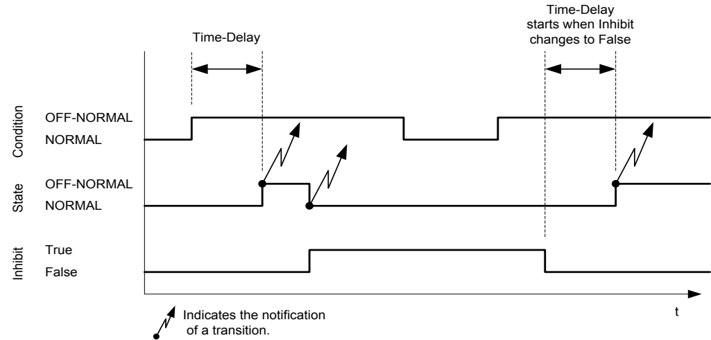
Figure 13-X4. Effect of Event_Algorithm_Inhibit on Event_State
