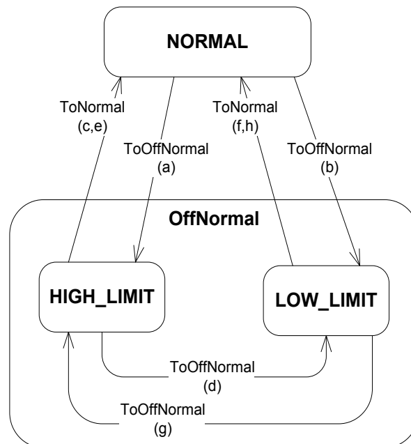
Figure 13-Y14. Transitions indicated by DOUBLE_OUT_OF_RANGE algorithm
