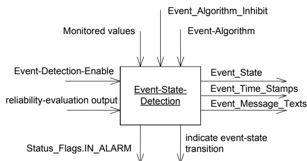
Figure 13-X2. The Event-State-Detection Process
