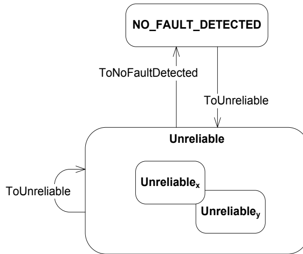
Figure 13-Y19. Transitions indicated by FAULT_EXTENDED algorithm
