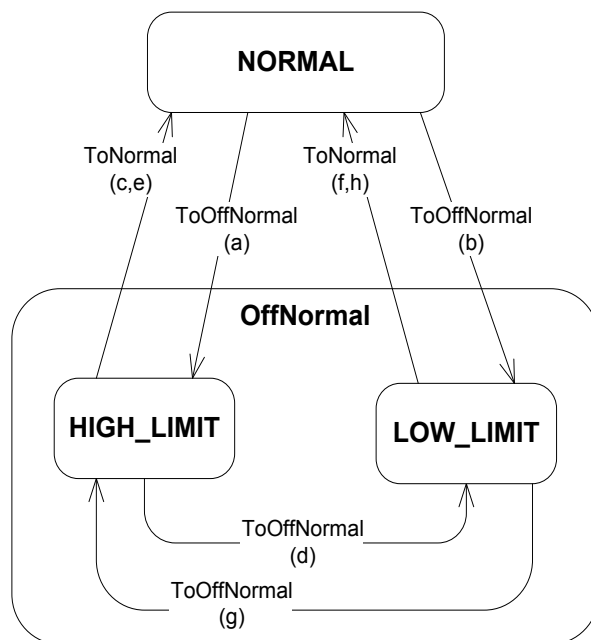
Figure 13-Y15: Transitions indicated by SIGNED_OUT_OF_RANGE algorithm
