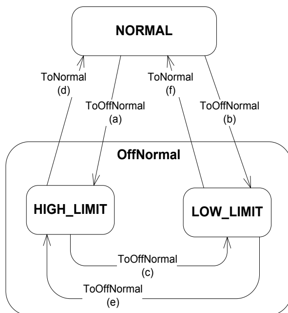
Figure 13-Y10. Transitions indicated by UNSIGNED_RANGE algorithm
