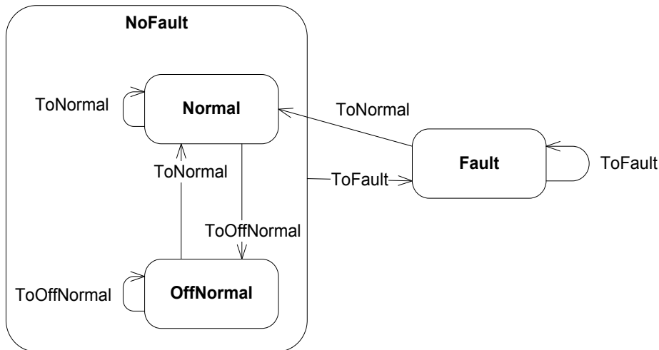
Figure 13-X3. Event-State-Detection State Machine
