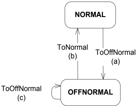
Figure 13-Y17. Transitions indicated by CHANGE_OF_CHARACTERSTRING algorithm
