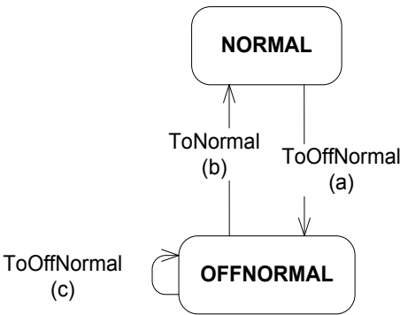
Figure 13-Y1. Transitions indicated by CHANGE_OF_BITSTRING algorithm
